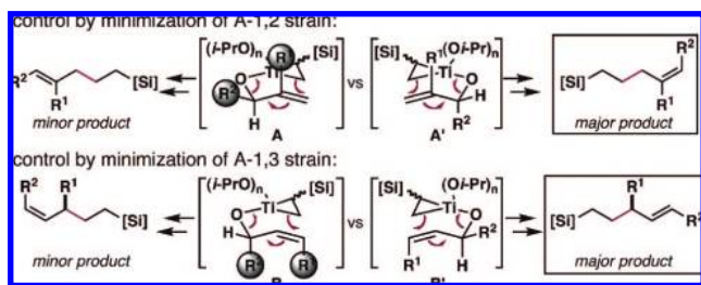
Figure 6. Model of stereoselection.
