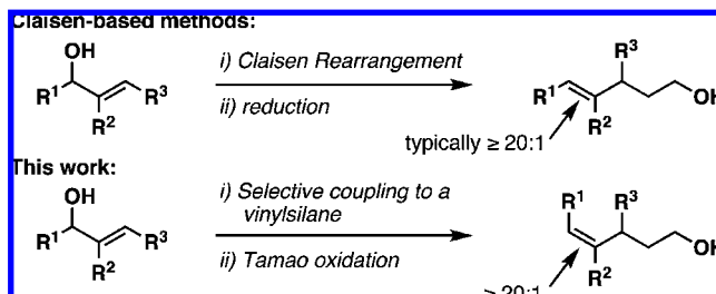
Figure 2. A stereochemically unique method for the synthesis of stereodefined trisubstituted alkenes from allylic alcohols.
