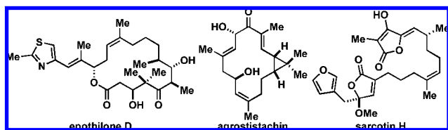
Figure 1. Natural products possessing stereodefined ( Z )-trisubstituted alkenes.
